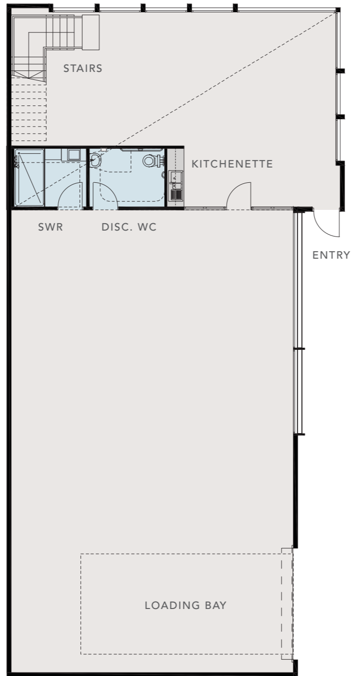
GROUND FLOOR
